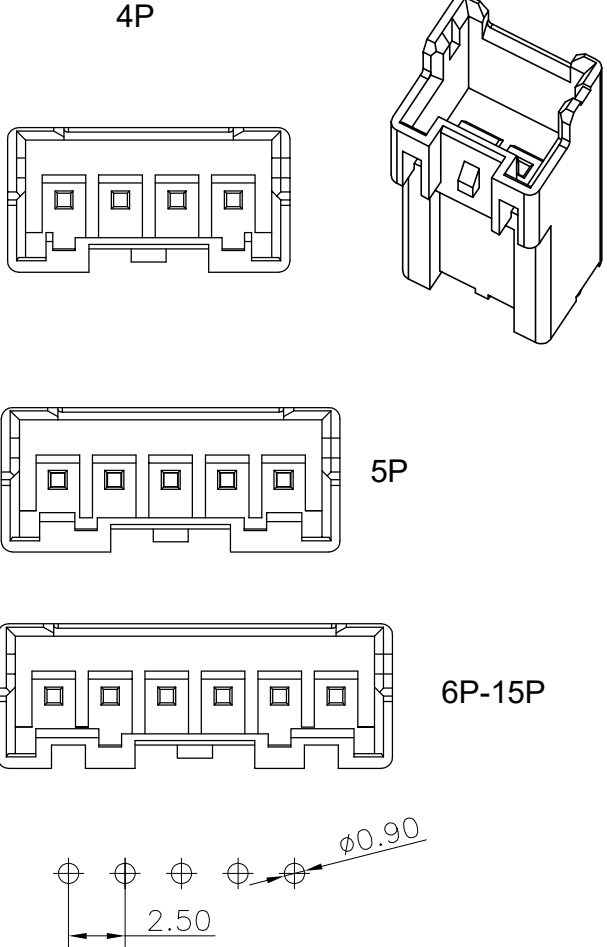
PCB LAYOUT
