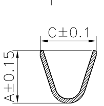
SECTION:A-A SCALE:1:1
