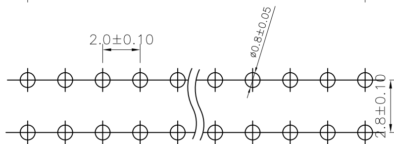
Recommended P. C. B. Hole Layout
