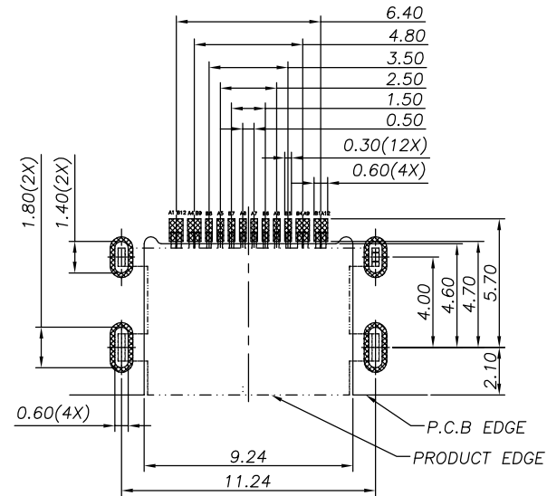
RECOMMENDED PCB LAYOUT(TOP VIEW) THICKNESS 1.20MM;DEFAULT TOLERANCE: \pm 0.05
