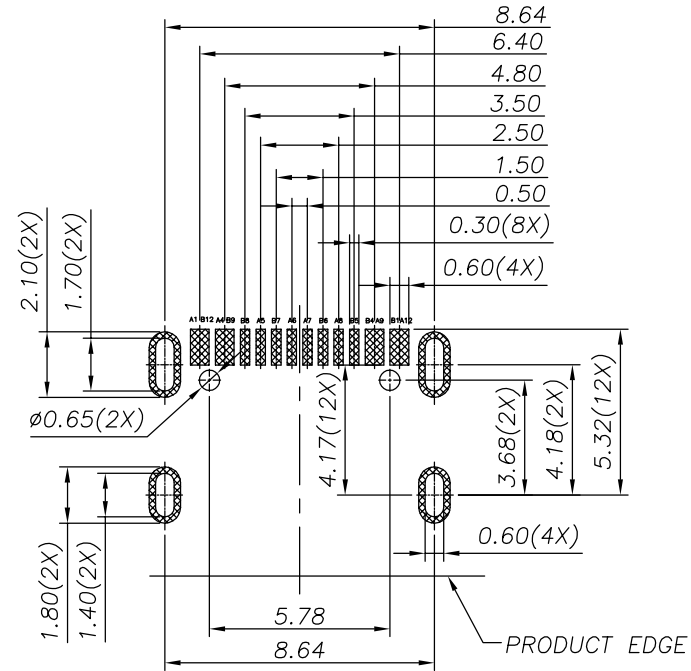
RECOMMENDED PCB LAYOUT(TOP VIEW) THICKNESS 0.80MM;DEFAULT TOLERANCE:±0.05
